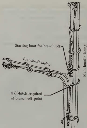
FIGURE 4-102. Lacing a branch-off.
